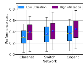
Fig. 11: The performance cost of normal packets misidentified by ProTO.
