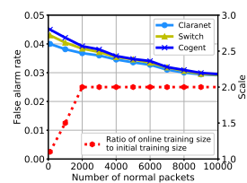
Fig. 7: False alarm rate for probe packet identification.
