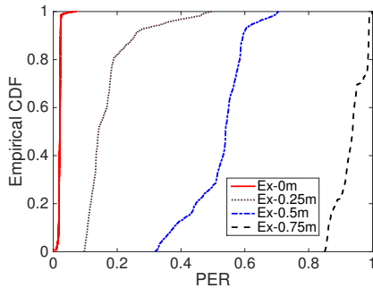
Fig. 7. Eavesdropper's PER.
